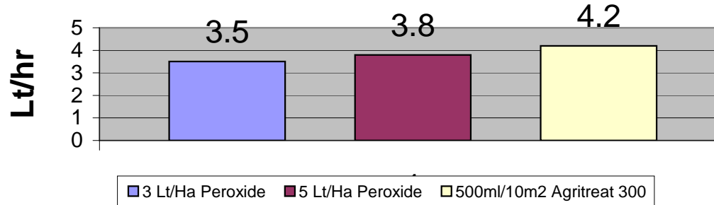
Bananas Komatipoort 4.2 Lt/Hr Eurodrip Compensated Drippers (one application)
